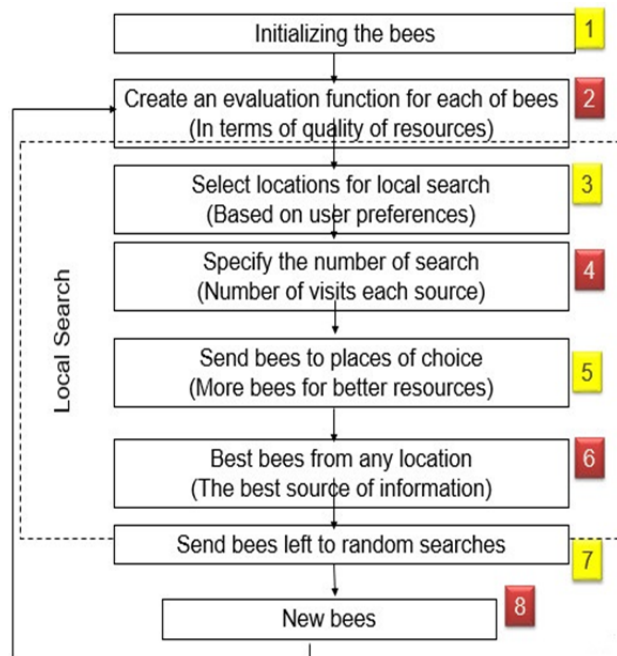
Figure 2. Bee colony algorithm proposed
